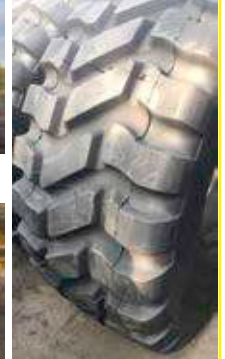
Goodyear 23.5R25, 2" Radial tyres, new, 43mm tread depth, TL3A+ E3/L3 Deep Latest production just in. Limited quantity available
